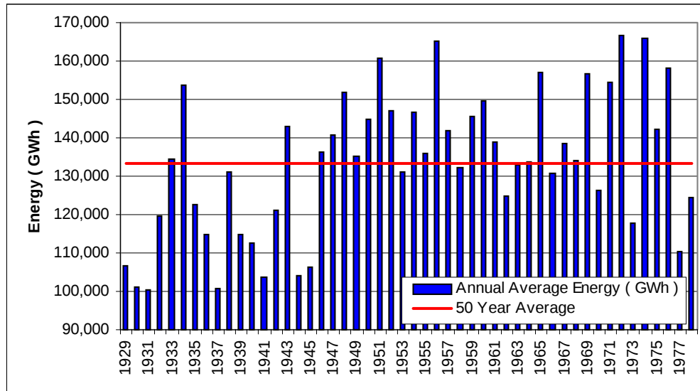
Figure 2-7: Annual Average Energy Available from Northwest Hydro Projects 1929-1978, GWh
